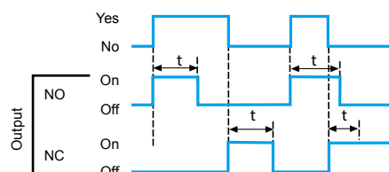
Monostable
